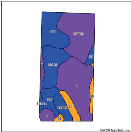
Soils Map
